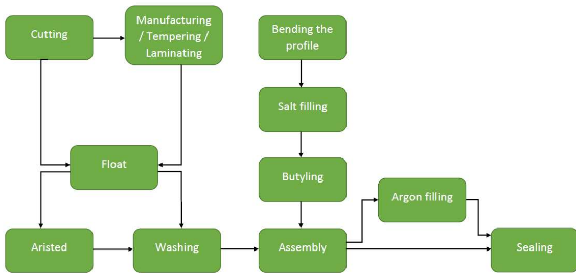
Figure 2. Manufacture process.
