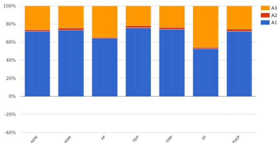
Graphic 1. Contribution by stages of composition Float de 4 mm // 16 // Templaranda de 4 mm
