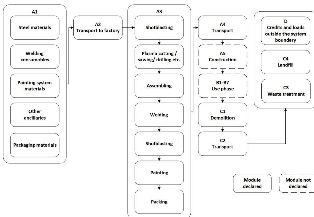
Figure 1: Overview of the production route of welded and painted steel structures (A1-A4, C1-C4, D)
