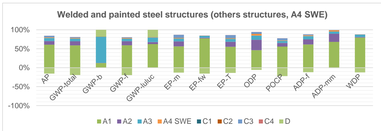
Figure 3: Influence of the modules on the environmental core indicators (other structures, A4 Sweden)
