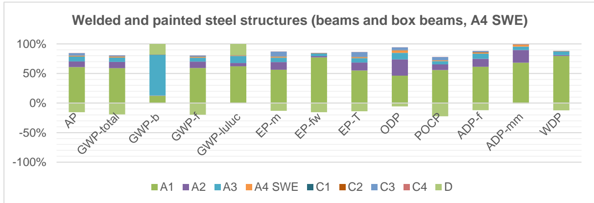
Figure 2: Influence of the modules on the environmental core indicators (box beams, A4 Sweden)
