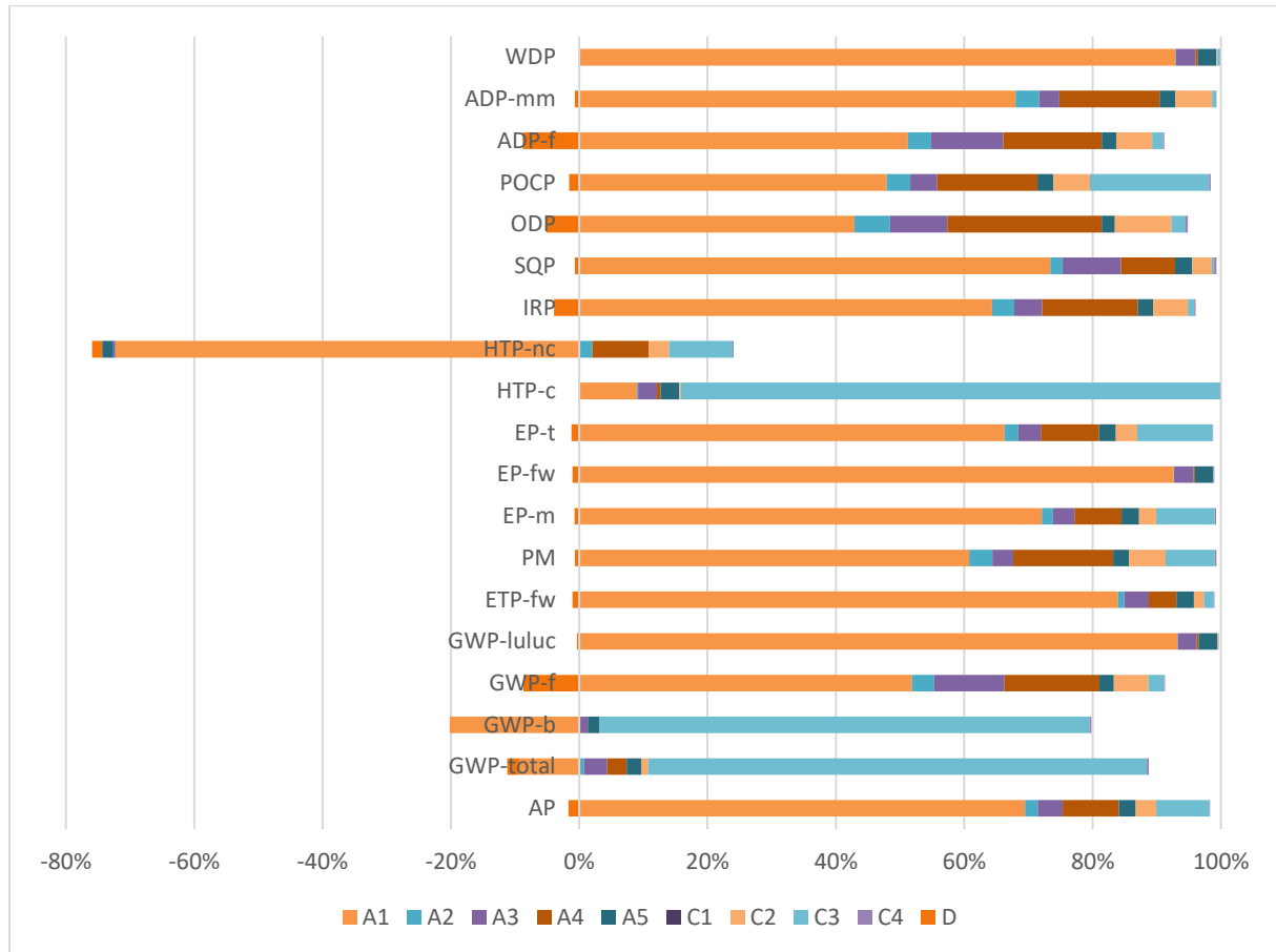
Figure 2: Shares of the product life phases in the environmental impacts for Jumpax® ME
