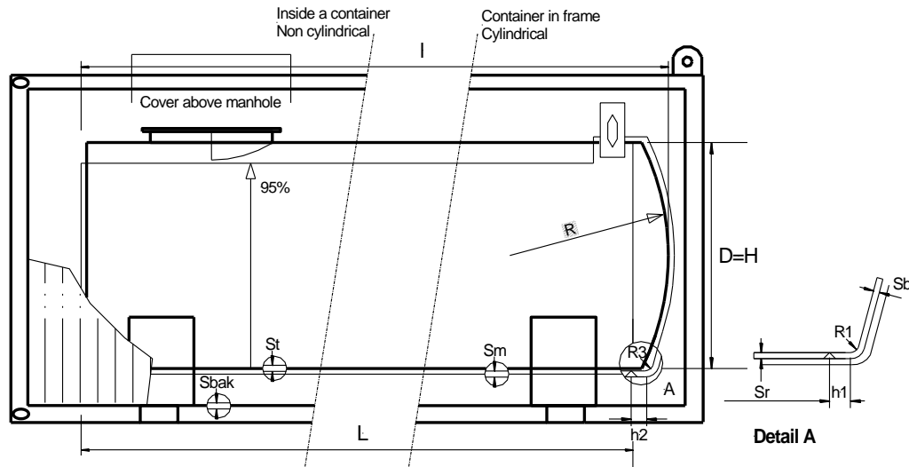
Figure Annex 8.1: Example tank container scope 1b
