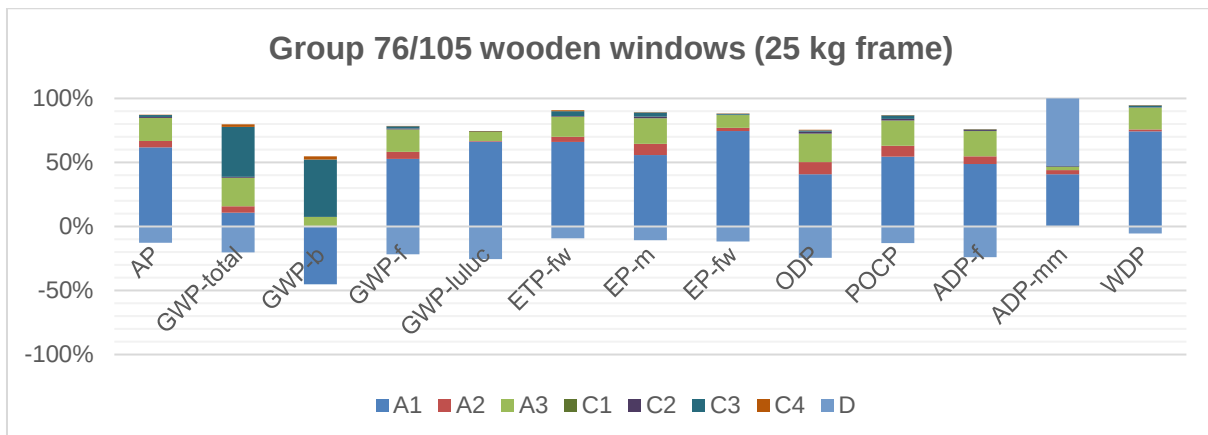
Figure 7: Influence of the modules A1 – A3, C1 – C4 and D on the analysed impact categories for 76/105 wooden window (frame 25 kg)
