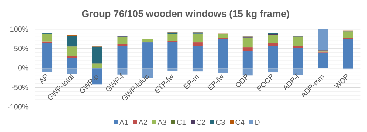
Figure 6: Influence of the modules A1 – A3, C1 – C4 and D on the analysed impact categories for 76/105 wooden window (frame 15 kg)
