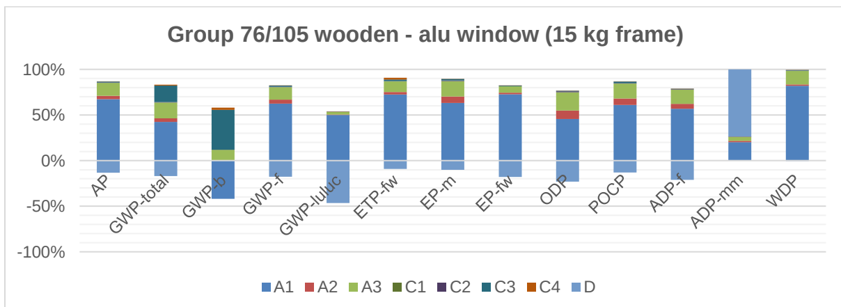
Figure 8: Influence of the modules A1 – A3, C1 – C4 and D on the analysed impact categories for 76/105 wooden – alu window (15 kg frame)
