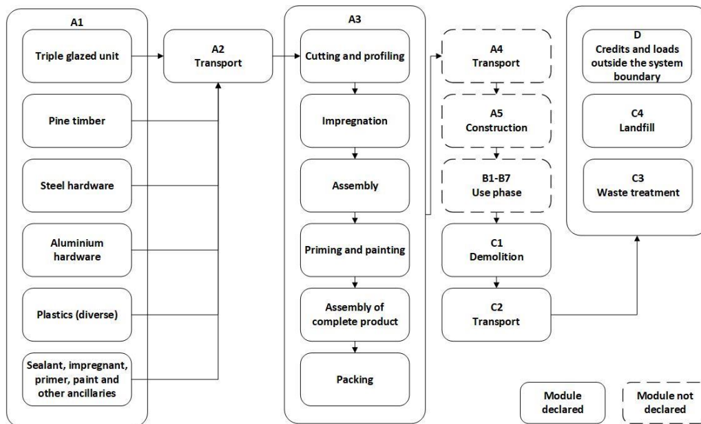
Figure 5: Overview of the production route of a window (A1-A3, C1-C4, D)
