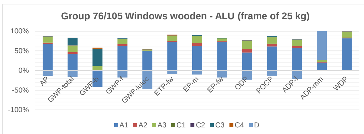
Figure 9: Influence of the modules A1 – A3, C1 – C4 and D on the analysed impact categories for 76/105 window wooden – alu (frame of 25 kg)
