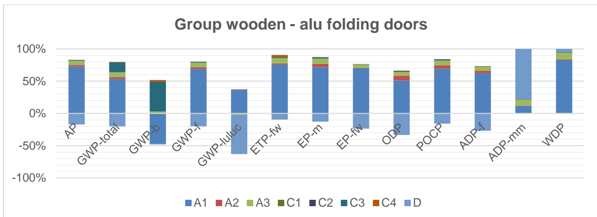
Figure 6: Influence of the modules A1 – A3, C1 – C4 and D on the analysed impact categories for wooden – alu folding door
