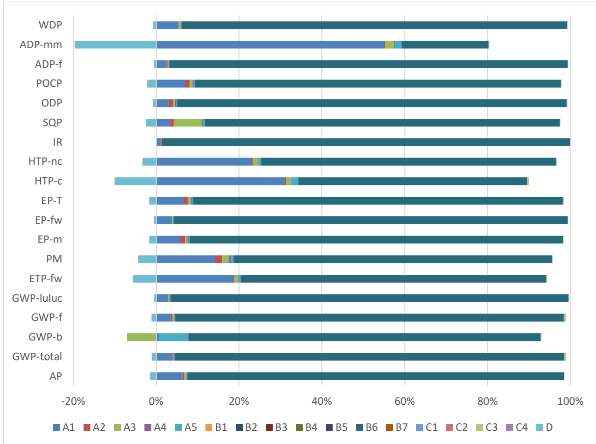
Figure 5: Percentage of the product phases in the environmental impact categories of aroTHERM plus 7 kW & Hydraulic Station
