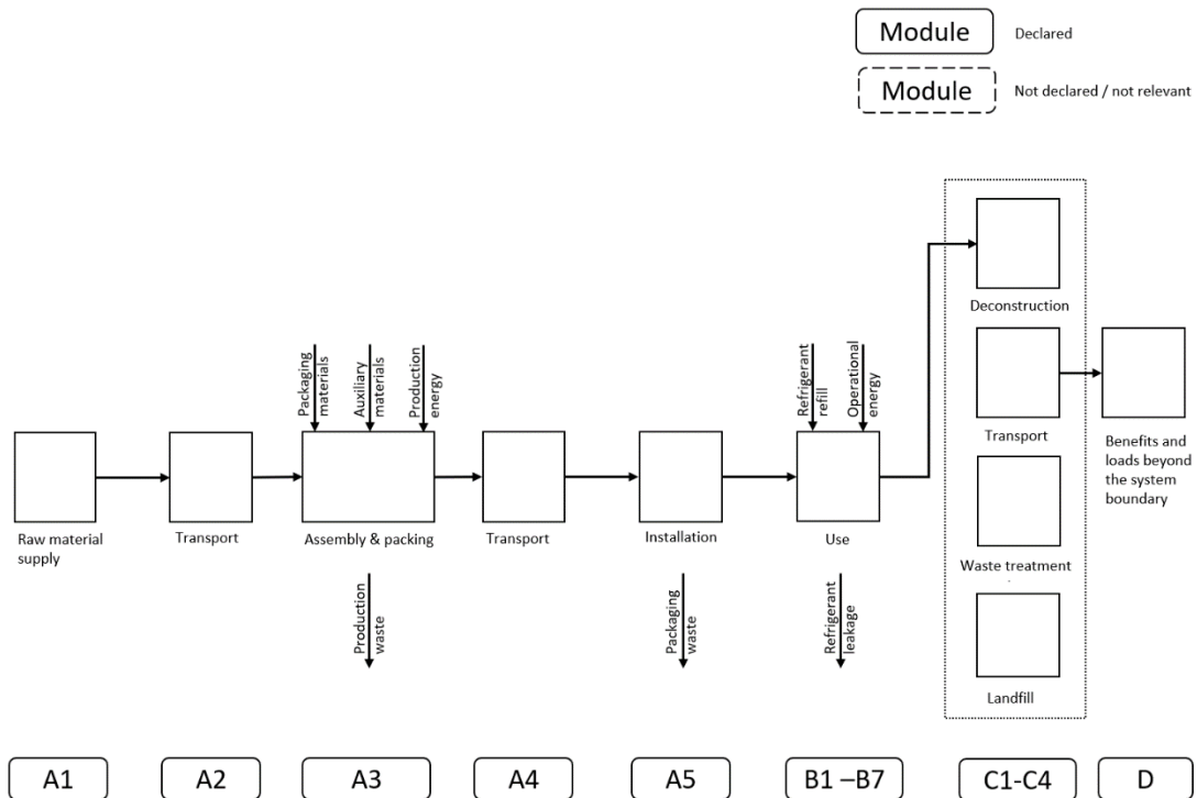
Figure 4: Process flow chart for aroTHERM plus 7 kW & Hydraulic Station
