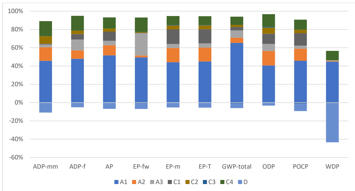
Figure 1: Influence of the modules on the environmental core indicators for type 44b
