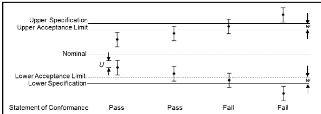
Figure 4 Graphical representation of a Binary statement with a guard band
