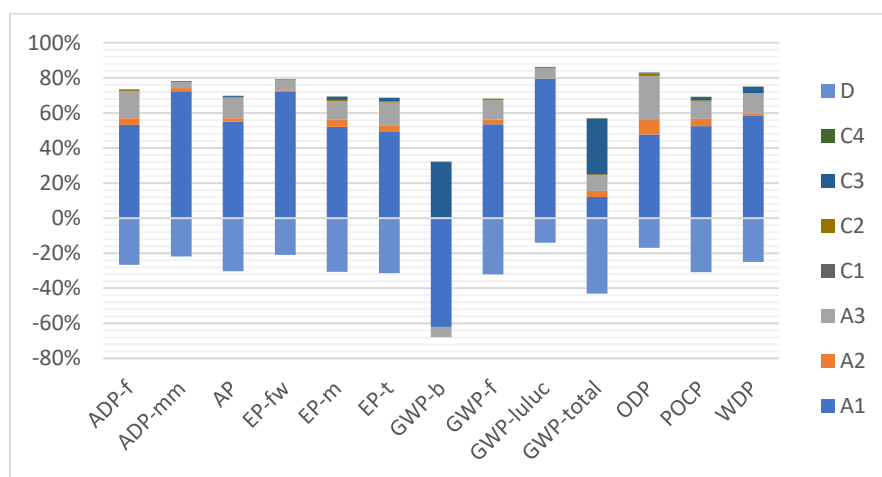
Figure 2: Influence of the information modules on the main impact categories – BYKO-DA55
