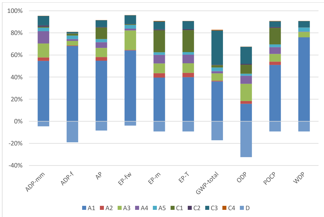
Figure 2: Tensar® InterAx® NX750-GD - Impact of the individual modules on the environmental core indicators (NMD set 2)
