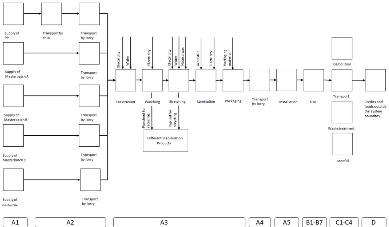
Figure 1: Process flow chart of the production of Tensar® InterAx® NX750-GD
