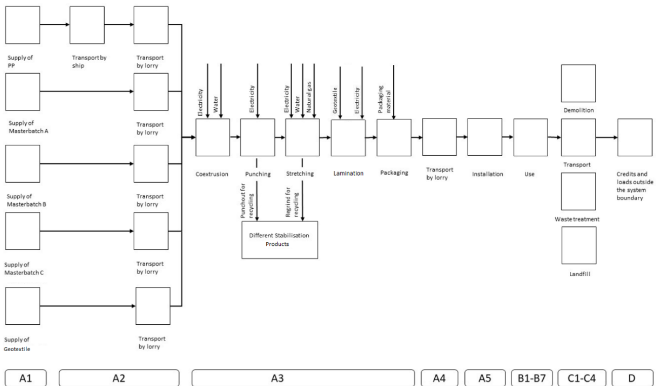
Figure 1: Process flow chart of the production of Tensar® InterAx® NX850-GD
