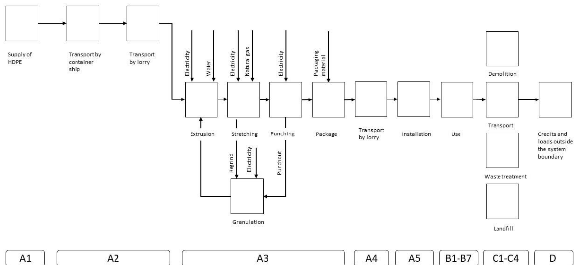
Figure 1: Process flow chart of the production of Tensar® ReAx RX2000
