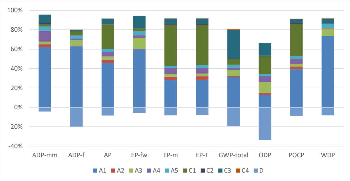
Figure 2: Tensor® TriAx® TX180 - Impact of the individual modules on the environmental core indicators
