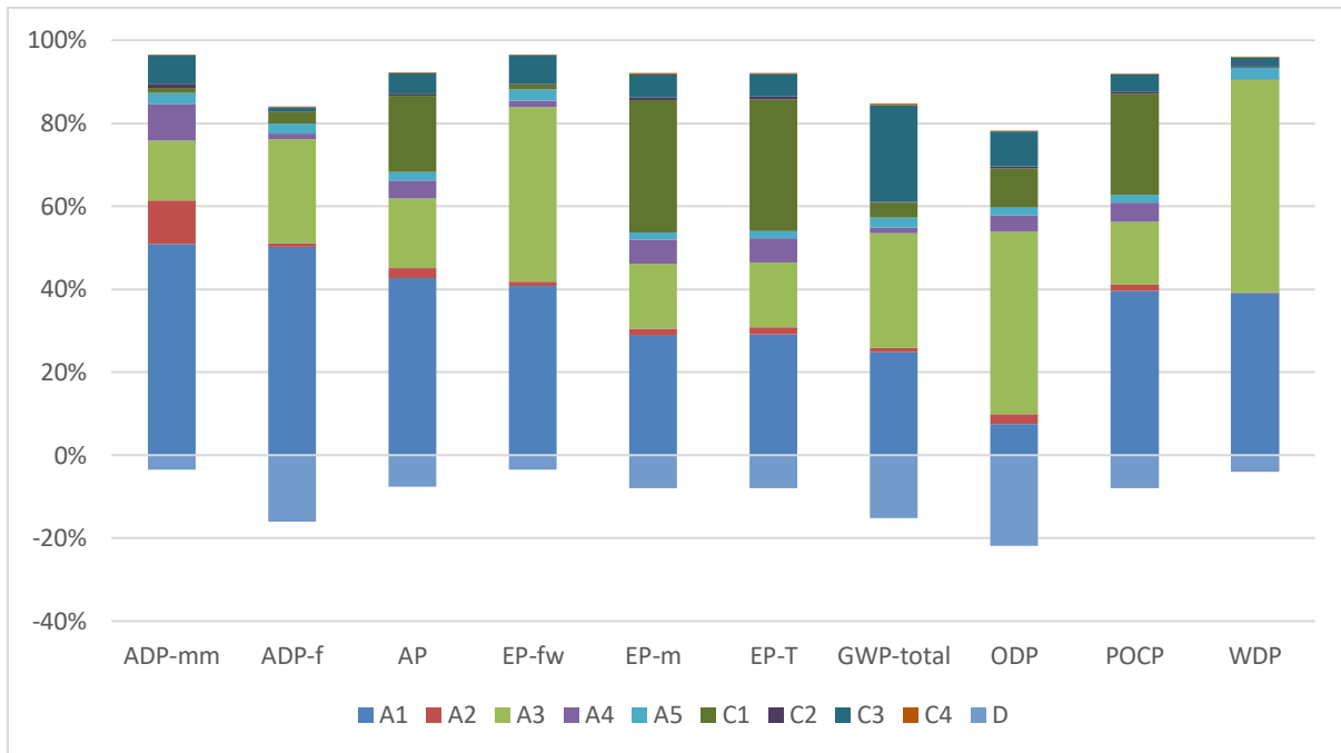
Figure 2: Tensar ® ReAx RX2600 - Impact of the individual modules on the environmental core indicator
