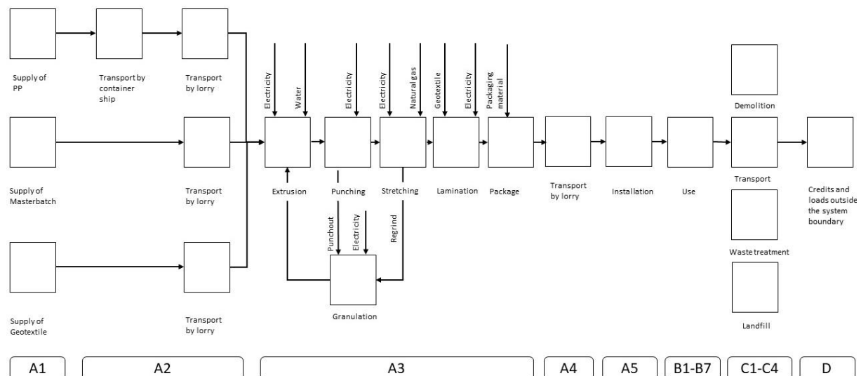
Figure 1: Process flow chart of the production of Tensor® TriAx® TX100-G series
