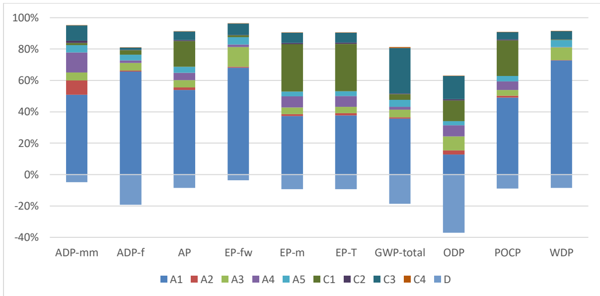
Figure 2: Tensor ® TriAx ® TX150L-G - Impact of the individual modules on the environmental core indicator
