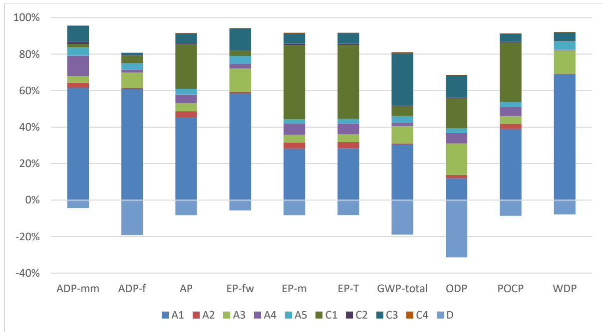
Figure 2: Tensar® TriAx® TX5 - Impact of the individual modules on the environmental core indicators
