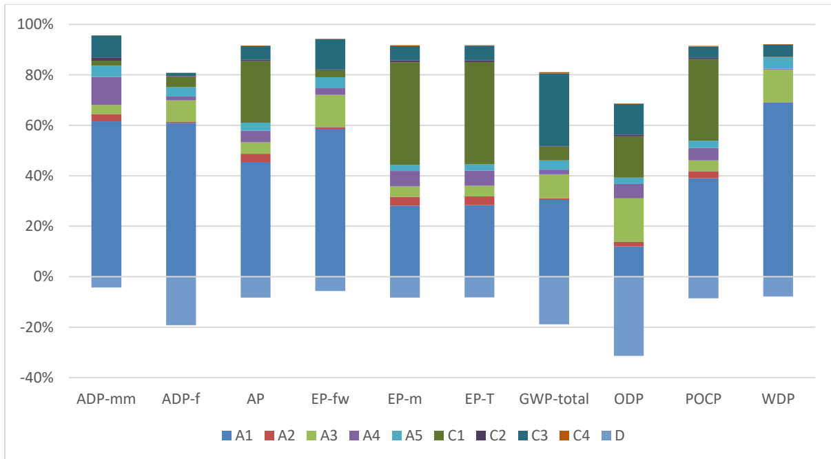
Figure 2: Tensar® TriAx® TX7 - Impact of the individual modules on the environmental core indicators
