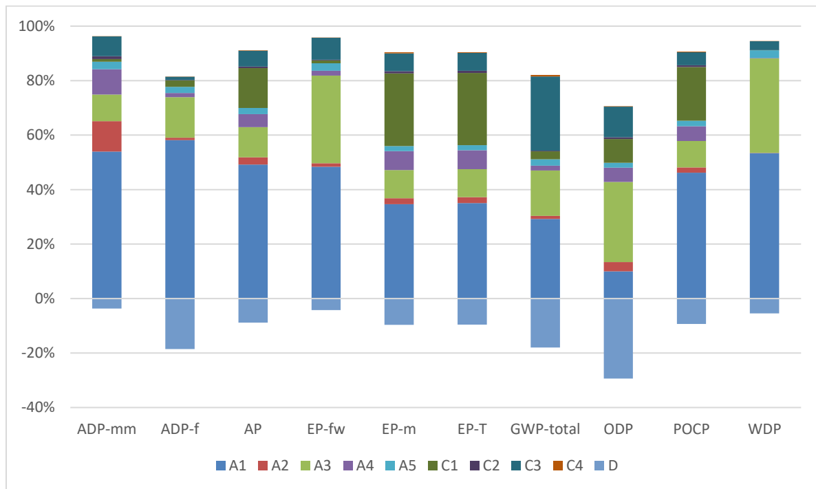
Figure 2: Tensar® RE580 - Impact of the individual modules on the environmental core indicators
