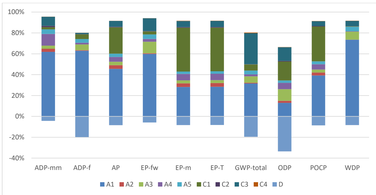
Figure 2: Tensar® TriAx® TX130S - Impact of the individual modules on the environmental core indicators
