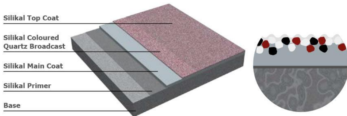
Figure 1: Composition System D Cold Floor
