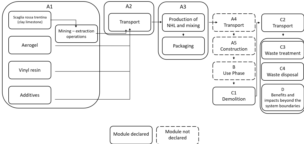
Figure 1: [Graphic schematic process flow diagram for the life cycle of VOLCALITE AIR PLUS.]
