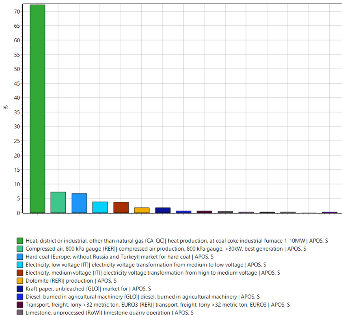
Figure 1: Relative contribution of the different inputs on the GWP of the NHL based adhesive for tiles.
