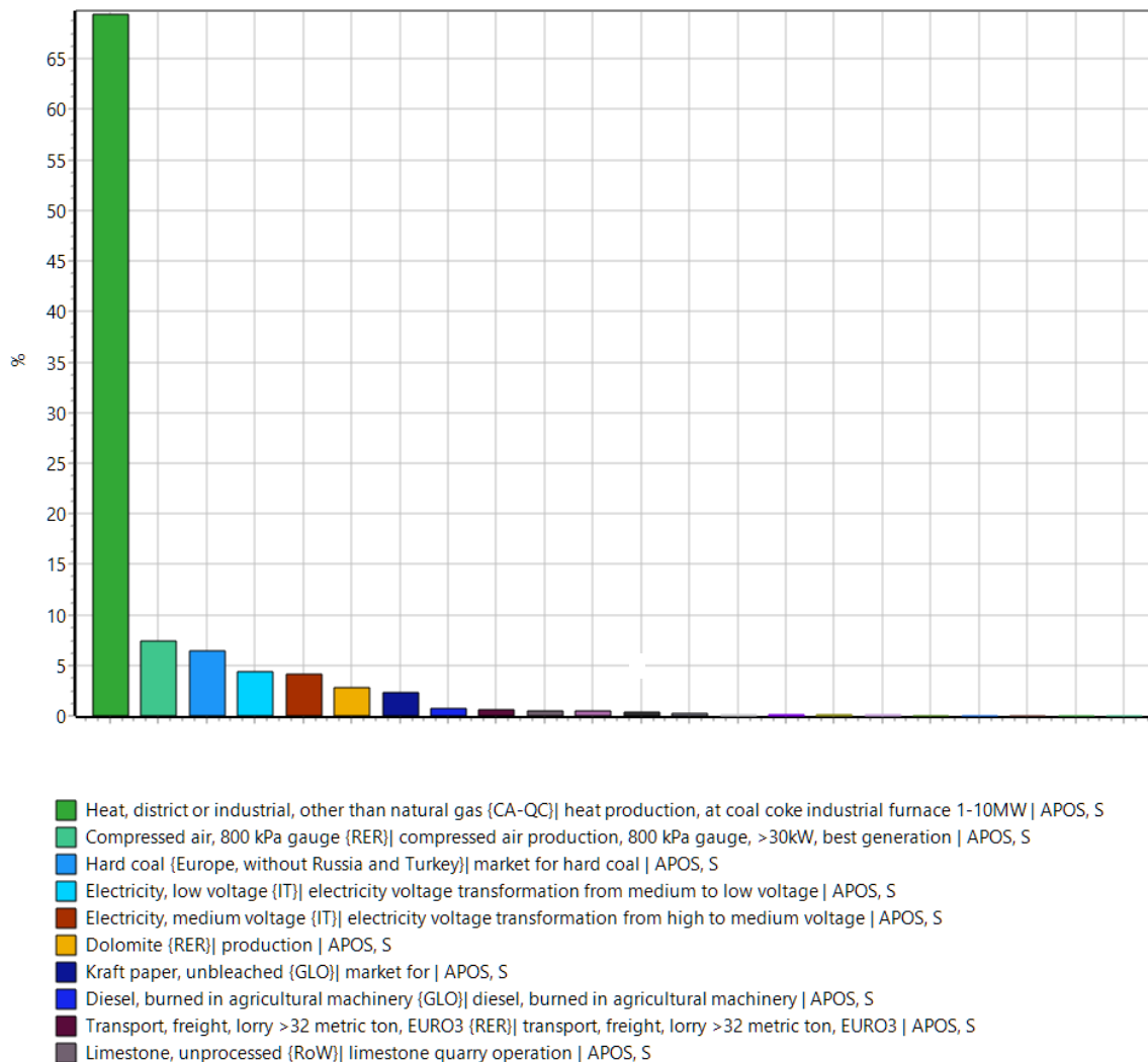
Figure 1: Relative contribution of the different inputs on the GWP of the NHL based adhesive.
