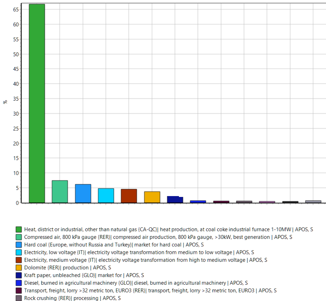
Figure 1: Relative contribution of the different inputs on the GWP of the NHL based mortar.
