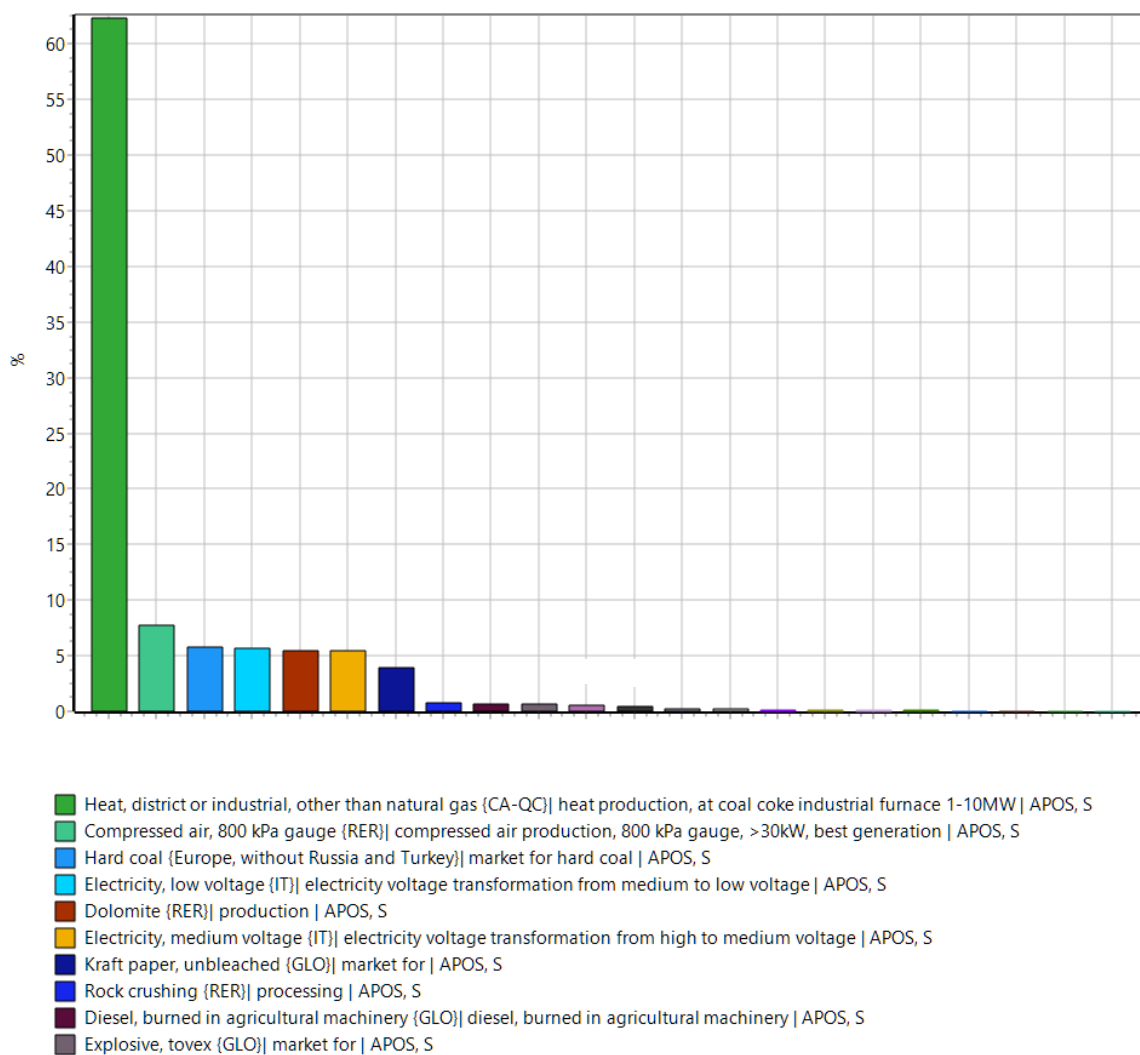
Figure 1: Relative contribution of the different inputs on the GWP of the NHL based screed floor.
