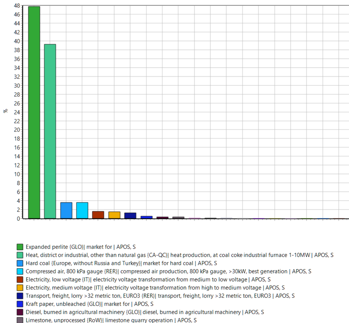
Figure 1: Relative contribution of the different inputs on the GWP of the NHL based light mortar.
