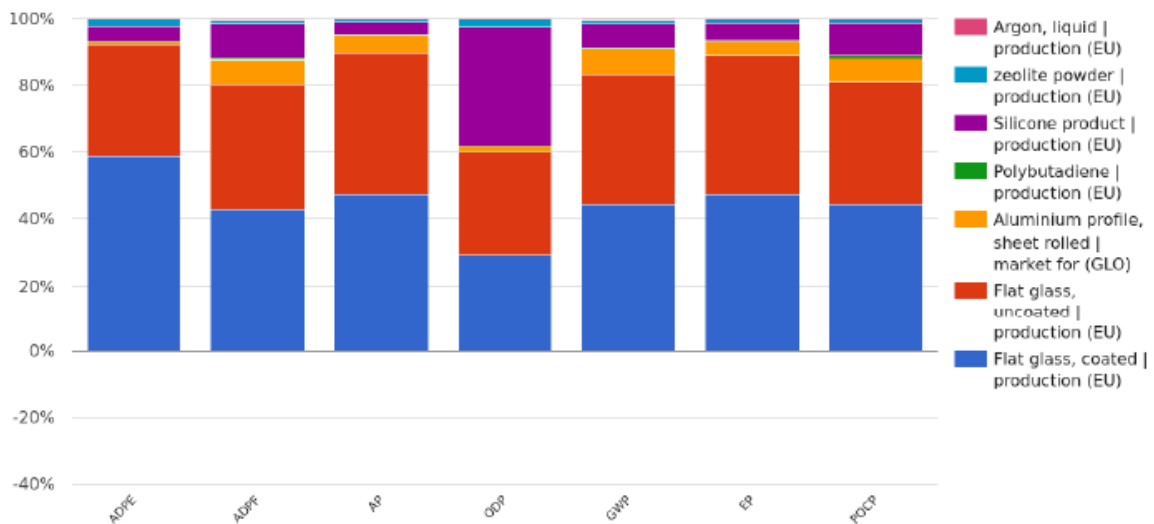
Graphic 2. Contribution of raw material to composition Float 6 template // 16 // Climaguard Premium2 6 template
