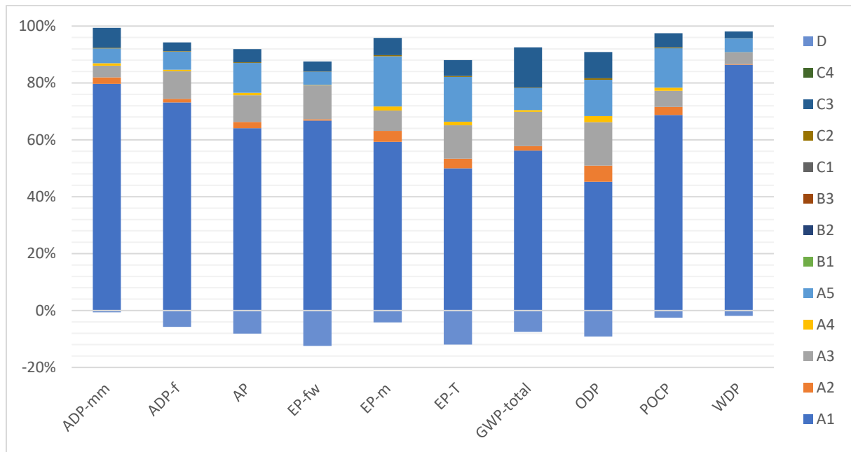
Figure 3: HaTelit® C40/17 - Impact of the individual modules on the environmental core indicator
