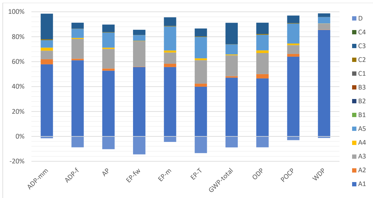
Figure 3: HaTelit® C40/17 eco - Impact of the individual modules on the environmental core indicator
