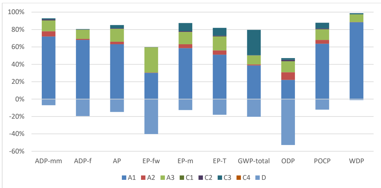
Figure 2: Head SL 235 - Impact of the individual modules on the environmental core indicators
