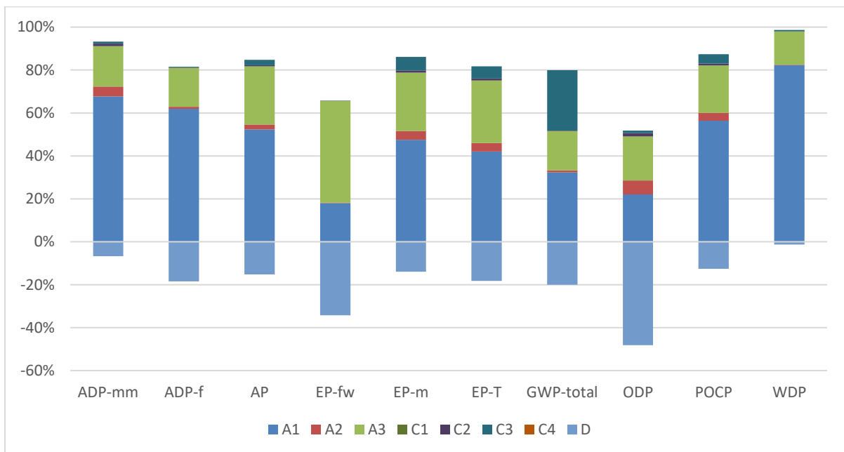
Figure 2: Head J 120 - Impact of the individual modules on the environmental core indicators
