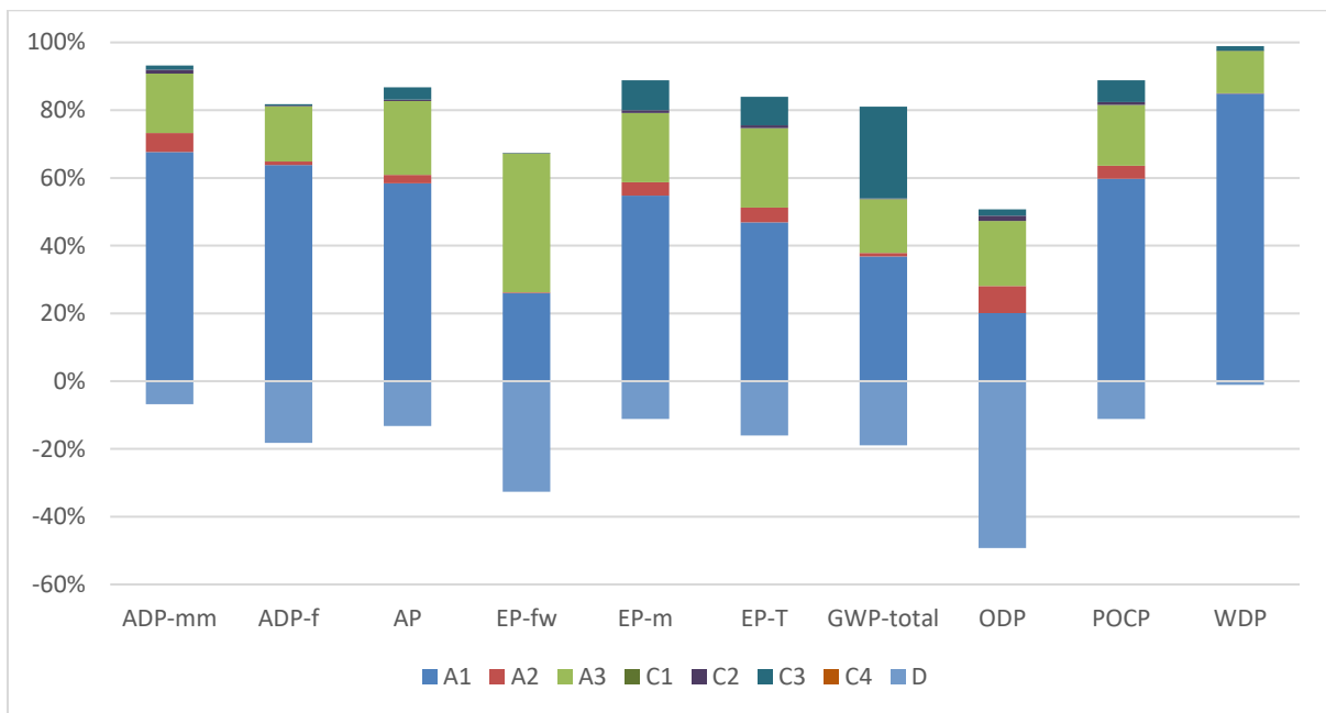
Figure 2: Head J 135/ 135 FH - Impact of the individual modules on the environmental core indicators
