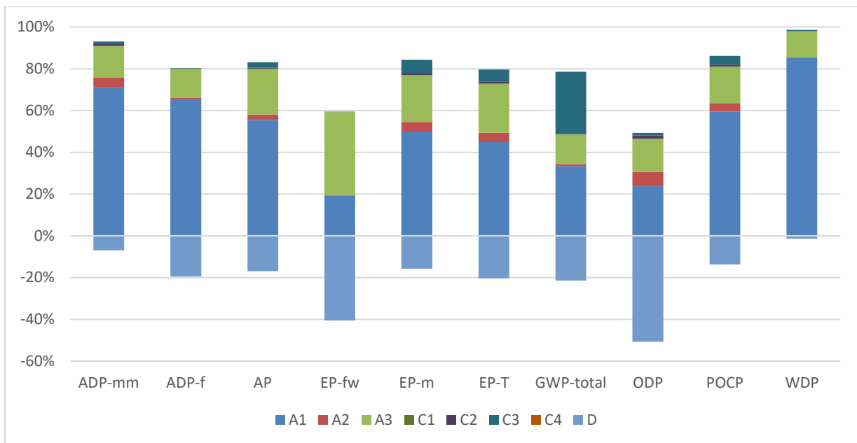
Figure 2: Head J 170 - Impact of the individual modules on the environmental core indicators
