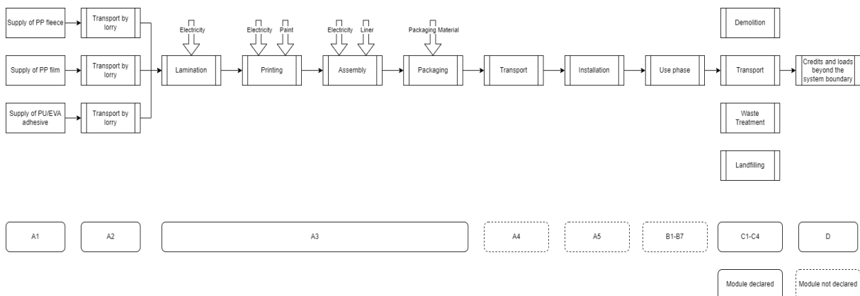
Figure 1: Process flow chart of the production of Head J
