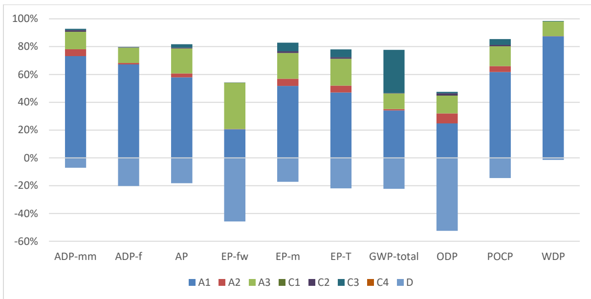
Figure 2: Head J 230 - Impact of the individual modules on the environmental core indicators
