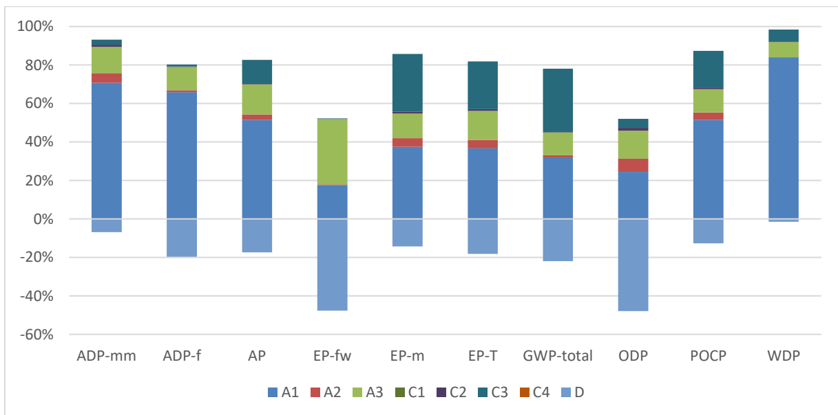
Figure 2: Head K 230 NV - Impact of the individual modules on the environmental core indicators
