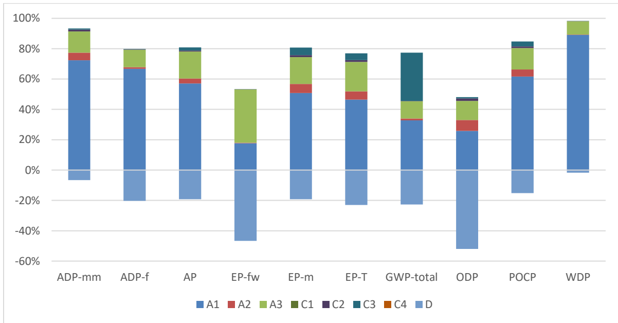
Figure 2: Head K 280 NV - Impact of the individual modules on the environmental core indicators
