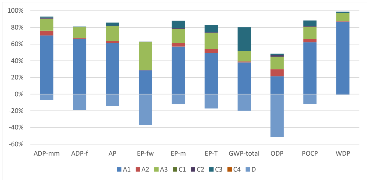
Figure 2: Head SL 185 - Impact of the individual modules on the environmental core indicators
