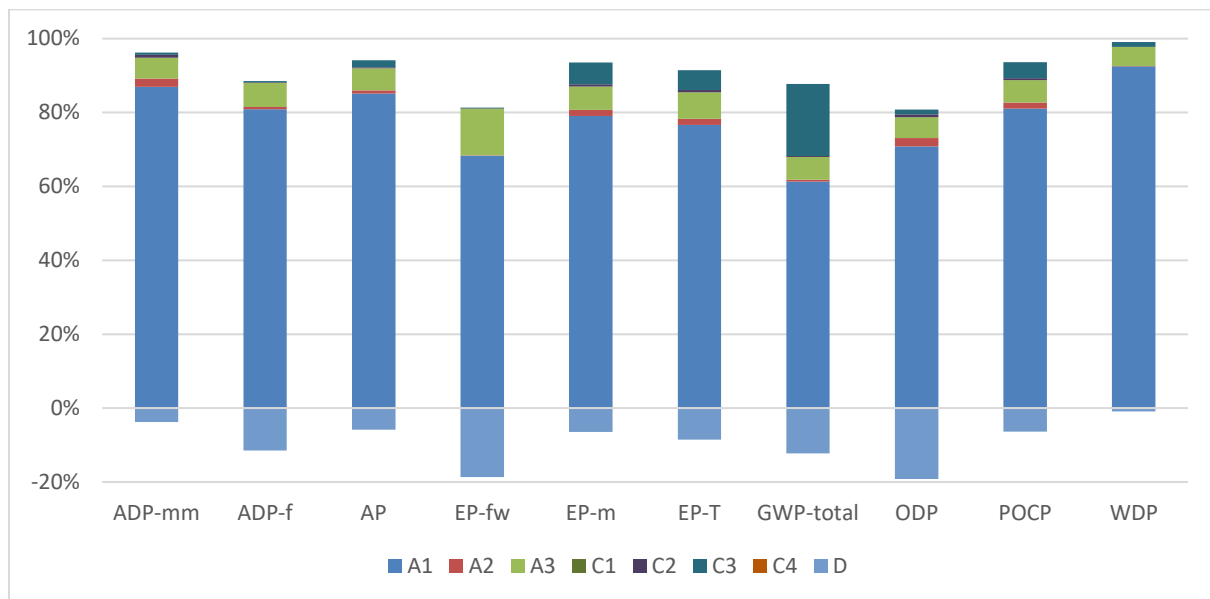
Figure 2: Head Protector Gold 330 - Impact of the individual modules on the environmental core indicators
