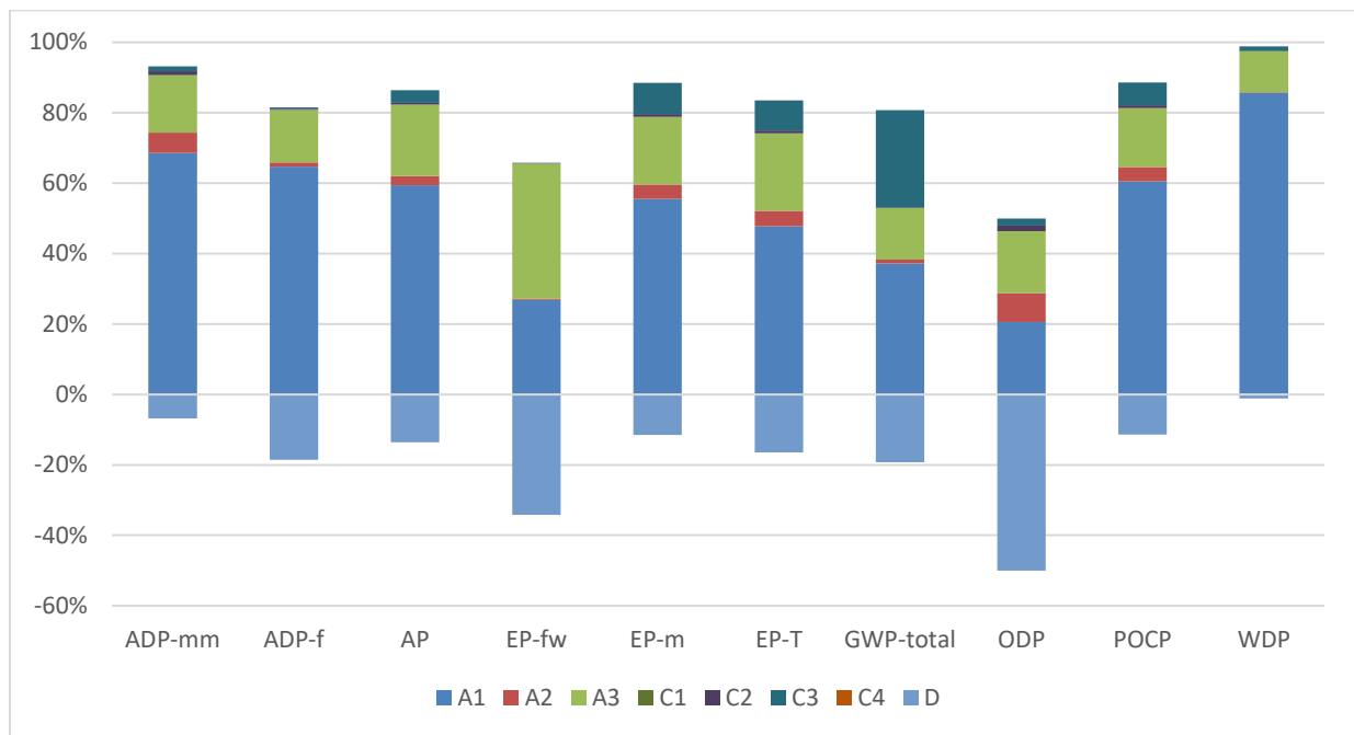
Figure 2: Head Protector FH 155 - Impact of the individual modules on the environmental core indicators
