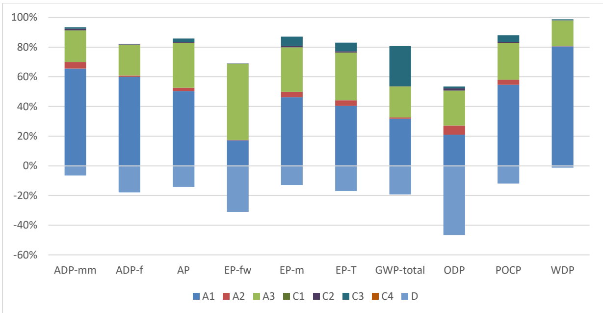
Figure 2: Syn Sd 20/100 - Impact of the individual modules on the environmental core indicators
