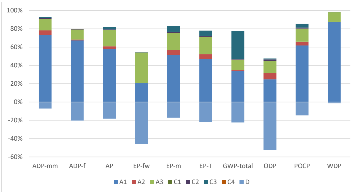
Figure 2: Syn J 230 Sd 20- Impact of the individual modules on the environmental core indicators
