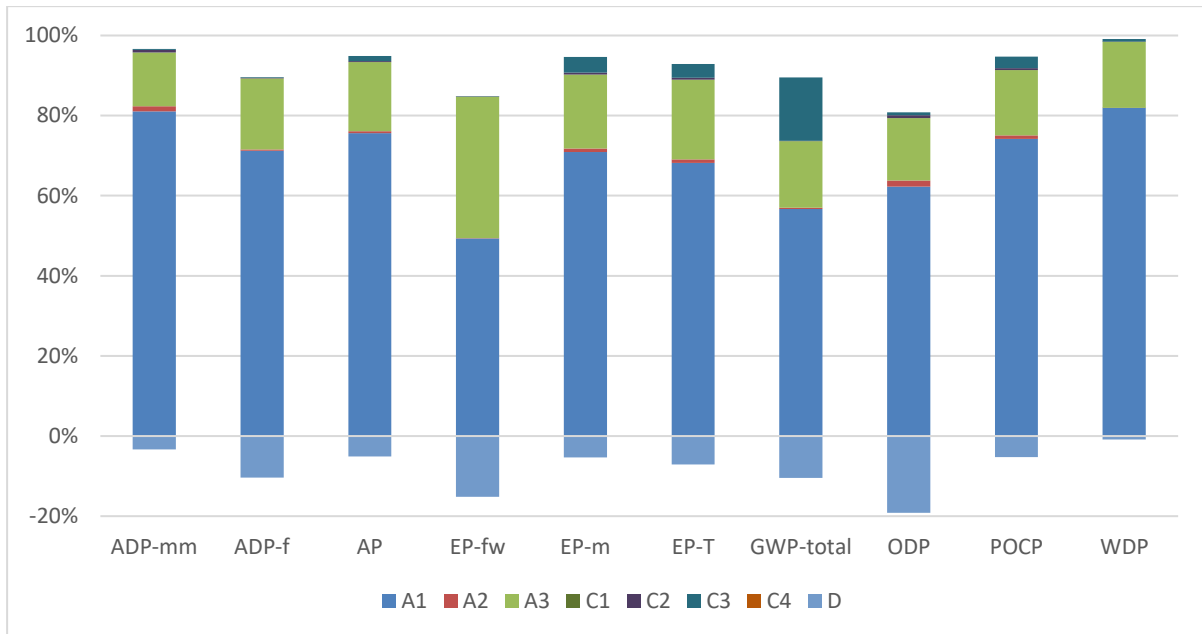
Figure 2: Syn Sd variabel 100 - Impact of the individual modules on the environmental core indicators
