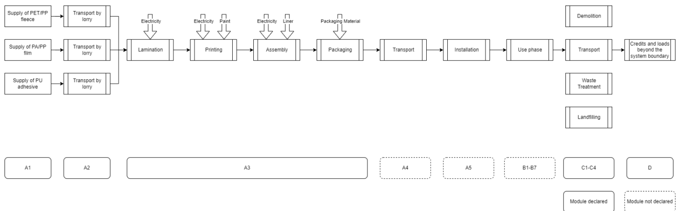
Figure 1: Process flow chart of the production of Syn Sd variabel 100
