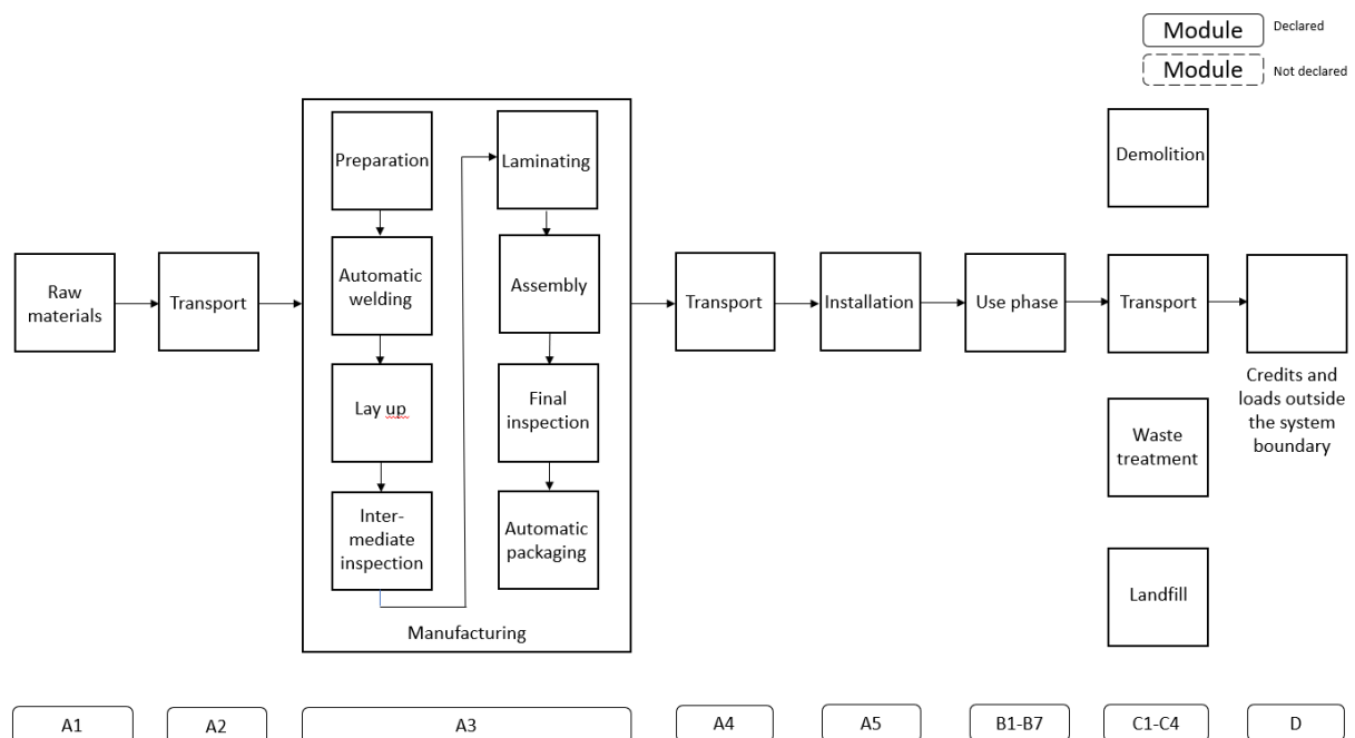
Figure 1: Process flow chart of the production of TWMNH-66HD.
