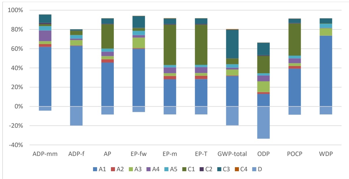
Figure 2: Tensar® TriAx® TXR - Impact of the individual modules on the environmental core indicators
