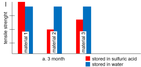
Fig. 2: Examples of corrosion after the storage of polymers in sulfuric acid: tensile strength of the material is an essential indicator of the corrosion process, as well as the possible occurrence of brittleness with the peeling off the coating (here pH: 1)
