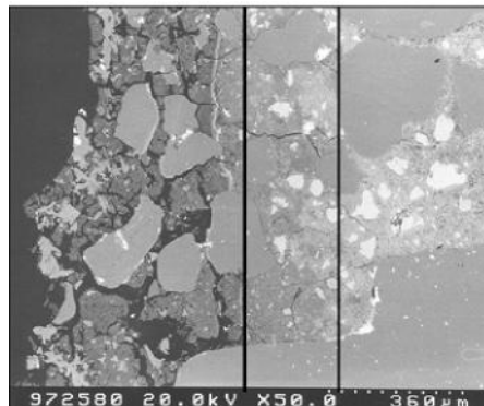
Fig. 6: 1st and 2nd damage front, determined on a thin grinding (SEM picture)
