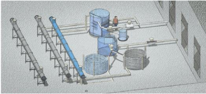
Fig. 3: 1 heating basin with heat exchanger | 2 fermenters | 3 free-flow pipe lines | 4 sample storage tank
