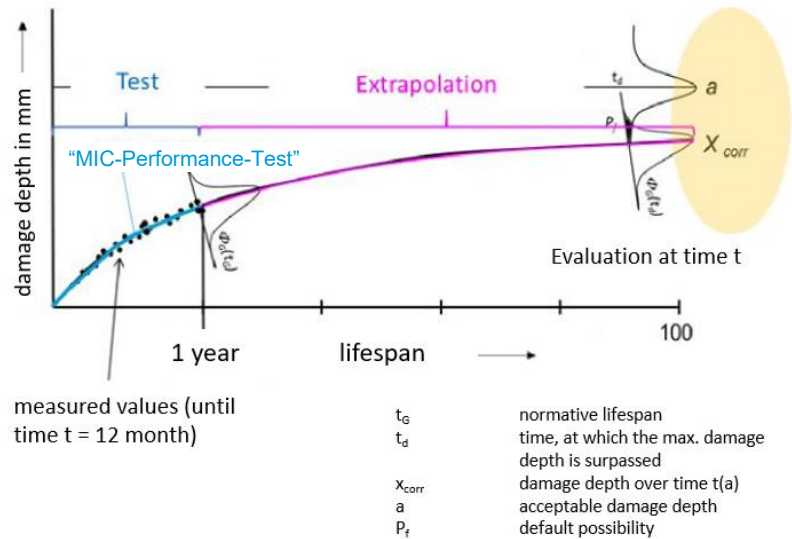
Fig. 7: Graphic representation of the damage depths up to 1 year Evaluation of the lifespan with a predetermined safety level
